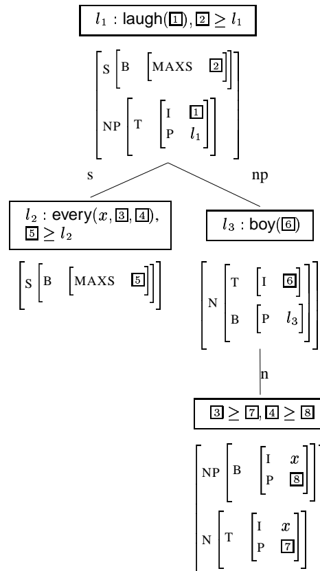
Figure 2: Semantics of (5) Every boy laughs .
